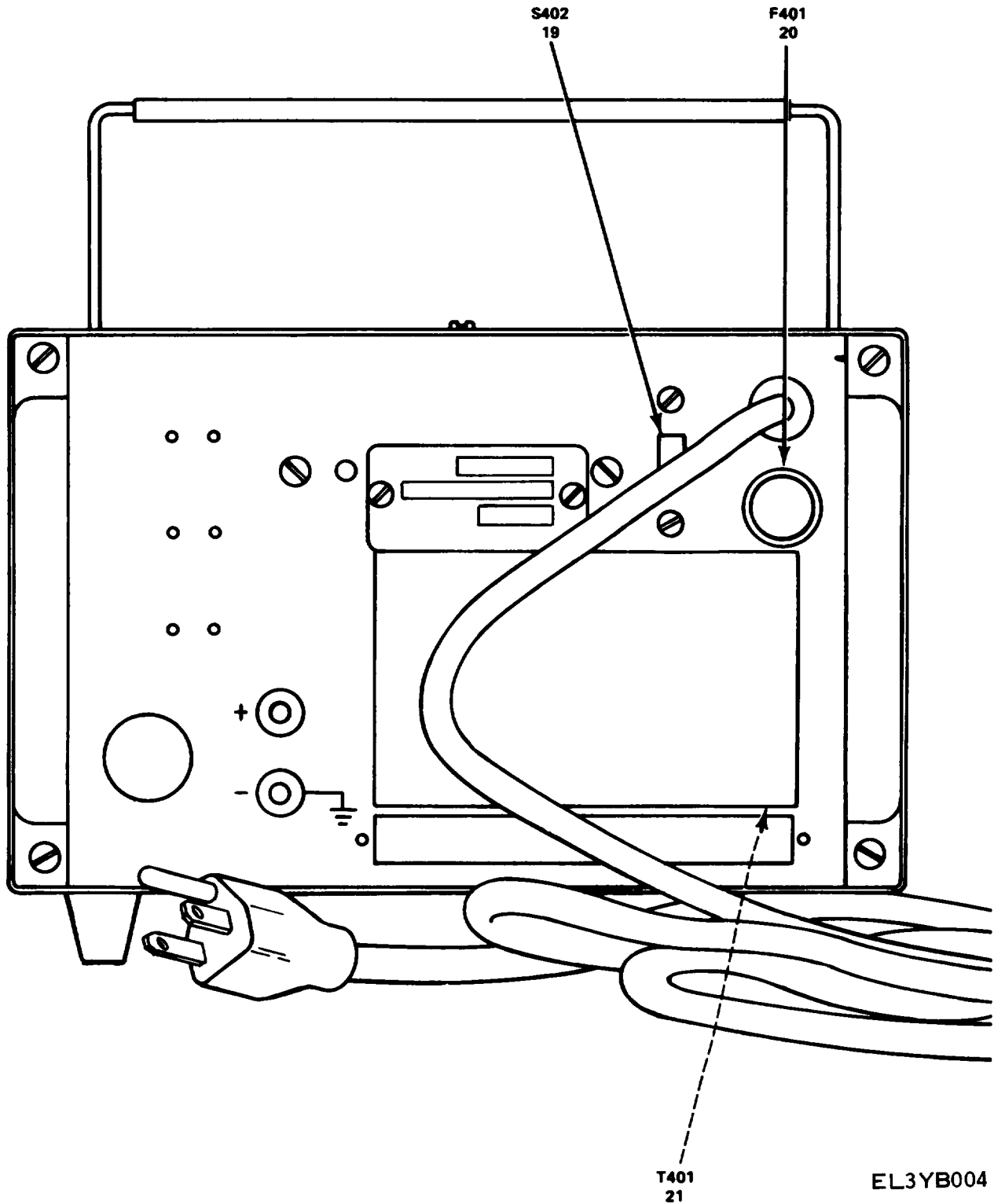
Figure 1. RF Power Meter, Boonton Model 42BD, Options 1 and 9 (Sheet 4 of 4).
