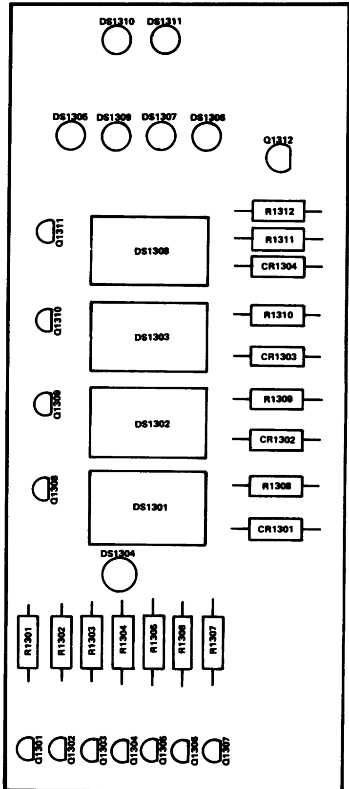
Figure 8. Circuit Card Assembly, Display, A8.
