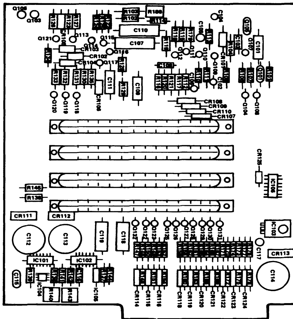
Figure 2. Circuit Card Assembly, Amplifier, A1.
